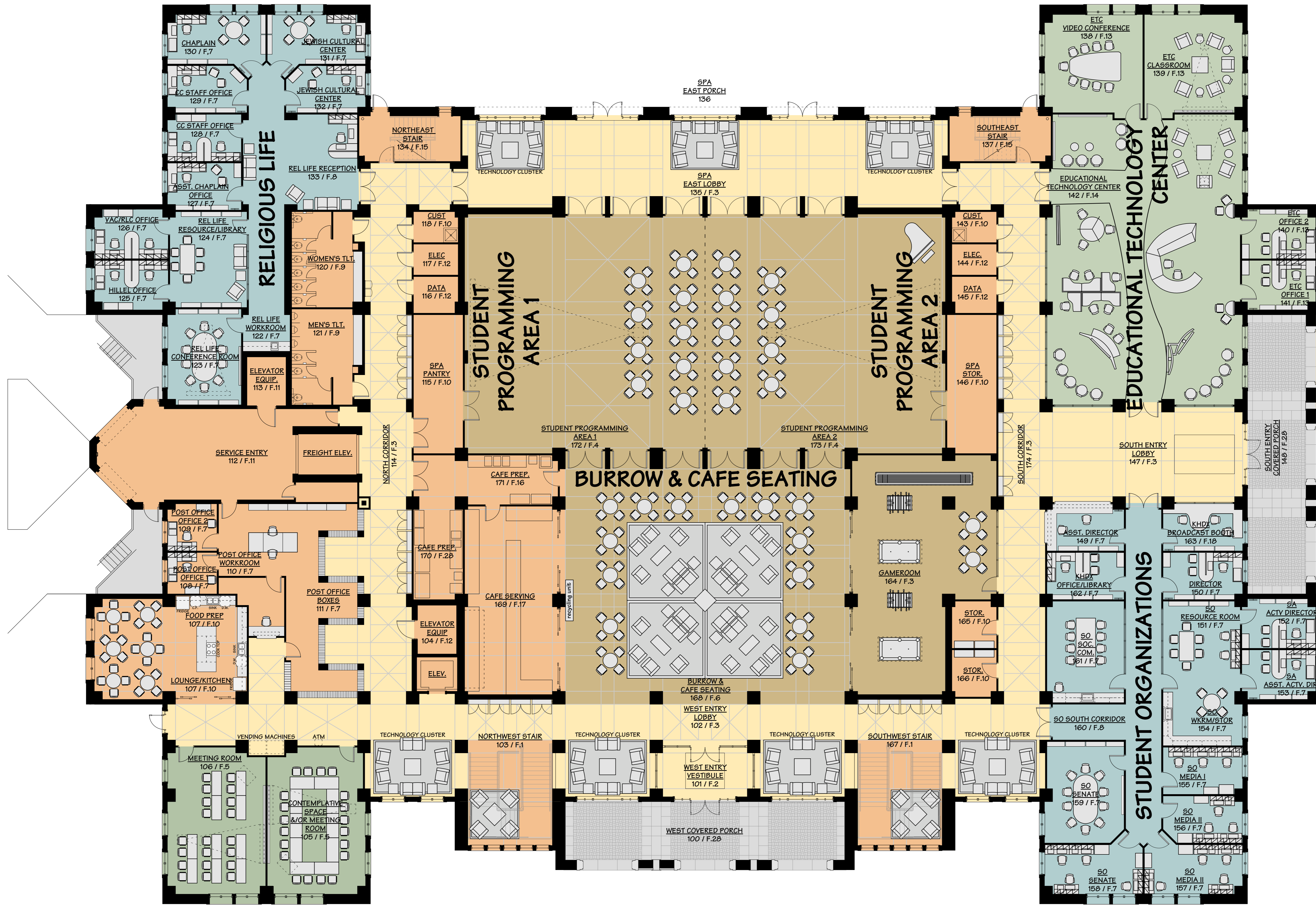
Hendrix College Student Life & Technology Center First Floor Plan - Kirchner Architecture, P.A. - 09.29.08
