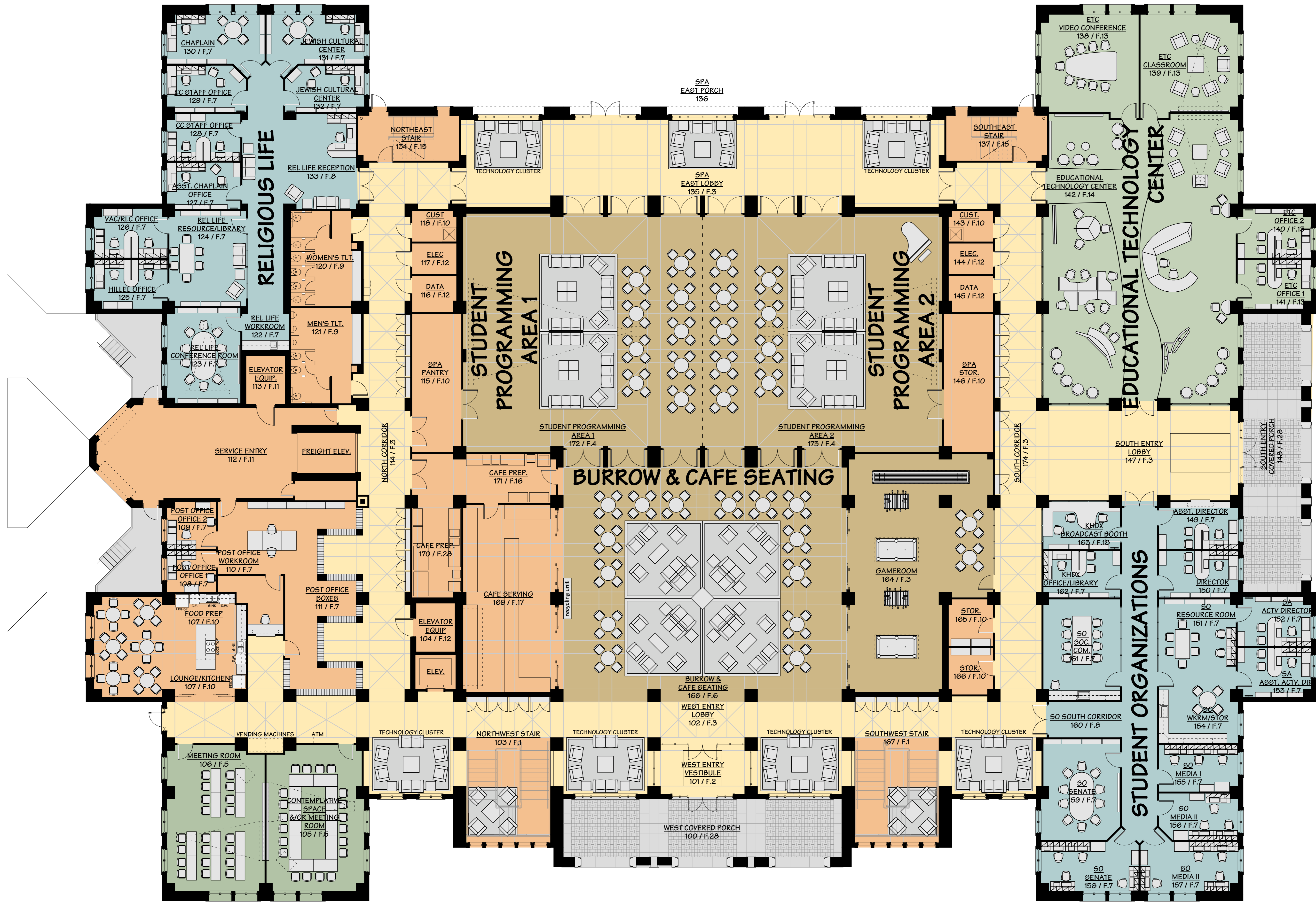
Hendrix College Student Life & Technology Center First Floor Plan - Kirchner Architecture, P.A. - 05.14.08
